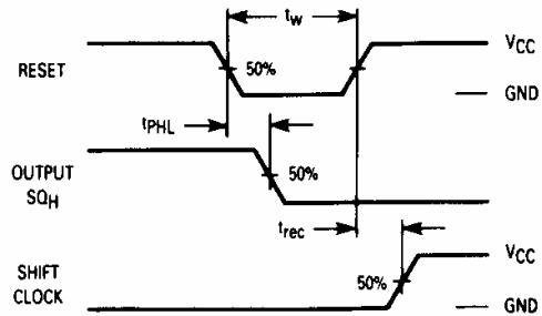
Figure 2. Switching Waveforms
